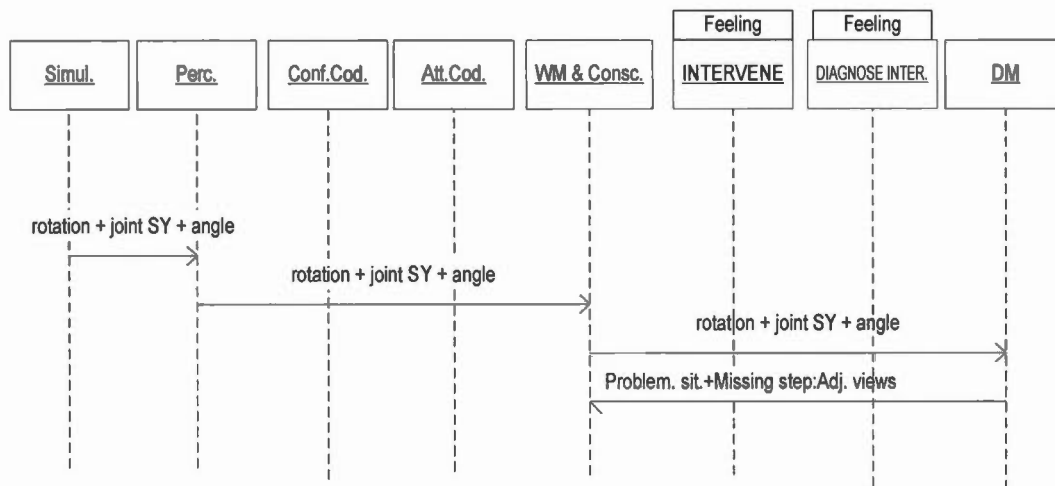
Figure 26 Incorrect procedure followed by the astronaut. The Domain Expert notices it and attempts to bring this to the attention of the Attention mechanism.
