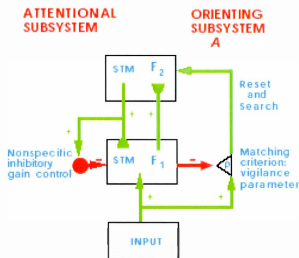
Figure 6 Fundamental principles of ART.
