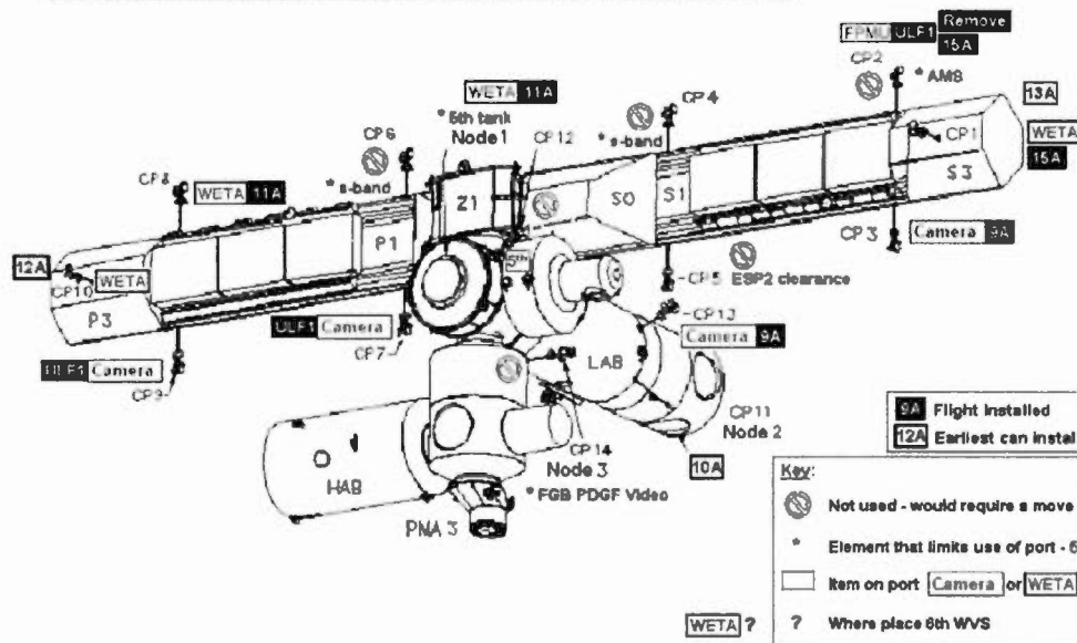
Figure 20 Location of the ISS camera ports that can connect installed cameras to Canadarm2 workstation. (Source: unknown)
