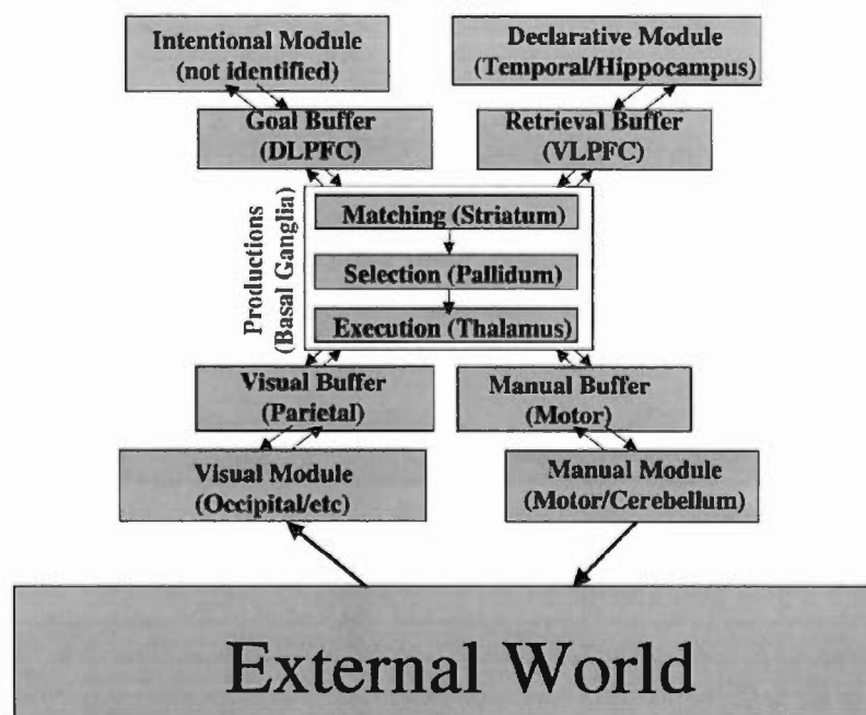
Figure 36 ACT-R's architecture. Source: Anderson et al., 2004
