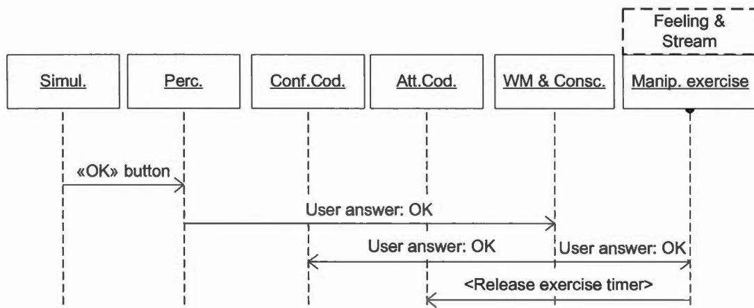
Figure 24 Portion of the initialization of a Canadarm2 manipulation exercise and noticing of inactivity by a "step timer" attention codelet.
