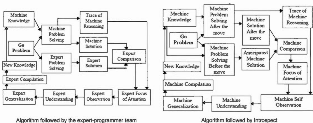
Figure 4 Comparison of developmental algorithm followed by the team of expert-programmers, and the one followed by Introspect.
