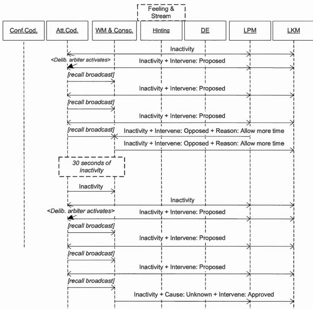
Figure 30 CTS deliberates about intervening and about the cause of user's inactivity. The conscious broadcast about the situation («Inactivity») brings the whole system to awareness but no cause is suggested. Nevertheless, some feelings get stimulated by this situation of inactivity, and readies the BN to react eventually. Just at the end of the standard deliberation duration, the LPM indicates its opposition to intervening without an explicit cause at this point in time: according to its beliefs about the astronaut, he probably just needs more time to think. After another waiting period, the same inactivity is signaled, but this time no one opposes an intervention.
