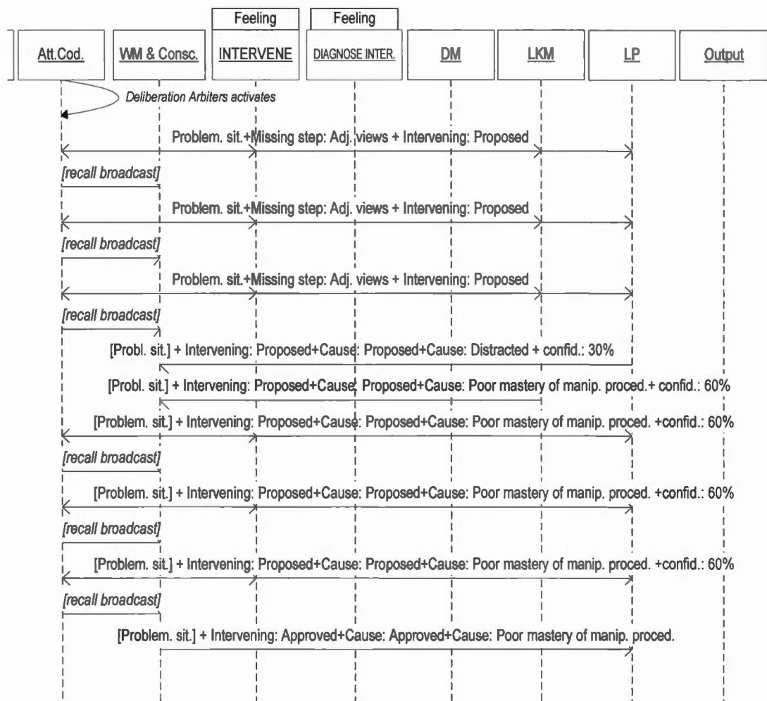
Figure 27 Intervening is proposed. As long as this is the most important coalition in WM, it gets published repetitively until the deliberation arbiter decides enough time has passed without any change (three cycles) or until causes are submitted. If more that one cause is offered, the Deliberation Arbiter chooses the most significant one and attaches it to the coalition under deliberation. If after a few cycles the cause proposed has not been opposed, the arbiter changes its status to «Approved».
