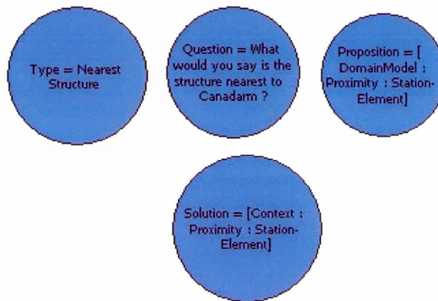
Figure 33 Behavior codelets that implement the question proposed by the Behavior node: «What would you say is the structure actually nearest to Canadarm?». The Domain Expert returns five names of modules to this specific request, which become the adapted answer choices presented to the user.
