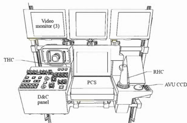
Figure 21 The ISS robotic workstation used to control Canadarm2. Source: NASA (2000) p.3-71.
