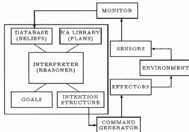
Figure 35 An agent implementing BDI principles: PRS. Source: Georgeff and Ingrand, 1989.
