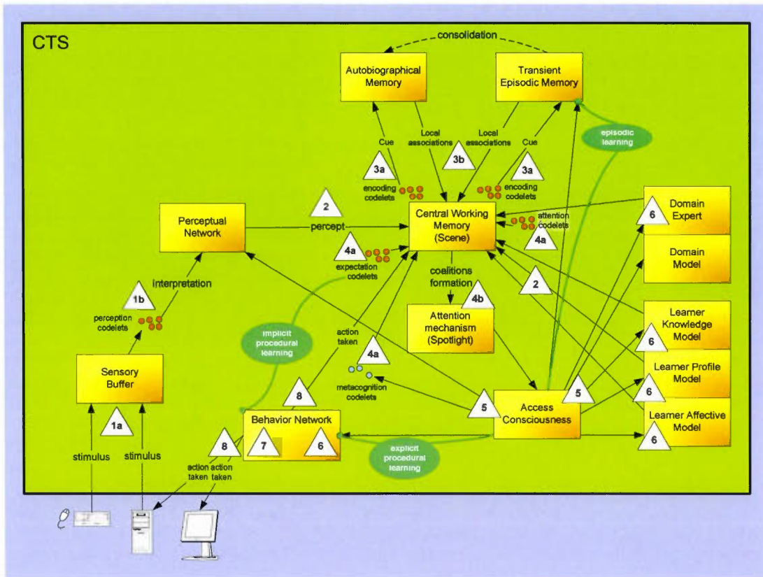
Figure 13 CTS' cognitive cycle. Although inherited from IDA, CTS' cognitive cycle presents originalities due to implementation differences (new modules, different implementations, different hypotheses). For instance, there is no instantiation in the Resource recruiting (6 th ) step.
