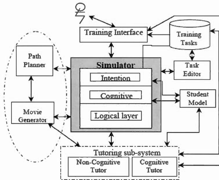
Figure 23 Architecture of Roman Tutor, cognitive version. Source: Nkambou, Belghith and Kabanza, 2006.
