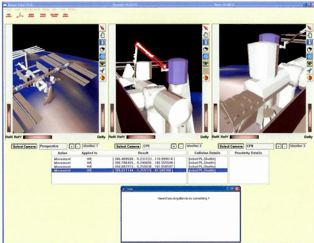
Figure 38 CTS reacts to an incorrect procedure. Here, the astronaut started moving Canadarm2 before creating all the necessary views on the three monitors. Admittedly, the help windows presented could use some polishing with choices like «No», «Why do you ask?». In any case, if the astronaut does not answer this message by adopting the needed corrections, CTS presents a more specific hint, then the plain fact, and, if nothing helps, the appropriate operation. Four levels of hints are the current remediation available.
