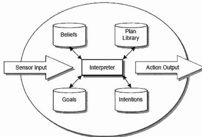
Figure 34 The BDI architecture. Source: d'Inverno, Kinny, Luck, Michael, et al. (1997).
