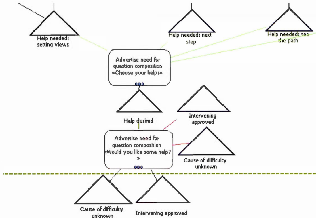
Figure 31 Beginning of the «Give general help» stream. It shares the precondition «Intervening approved» with the «Hinting» stream, but has the unique precondition «Cause of difficulty unknown». This stream gets involved when no module could suggest a cause to the situation. In this situation, CTS needs to interact with the user to find how it can help in what it believes to be a problematic situation.
