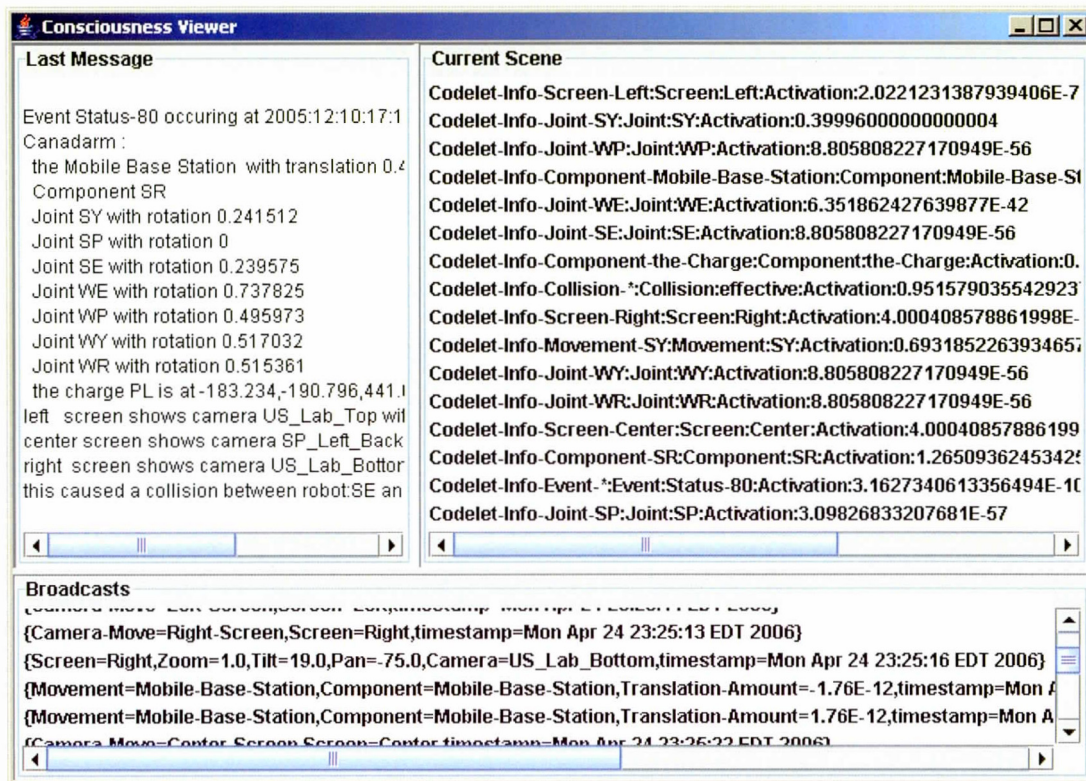
Figure 15 The Consciousness Viewer , a simple but very useful extension of the Global Workspace class, for comprehension and debugging needs.
