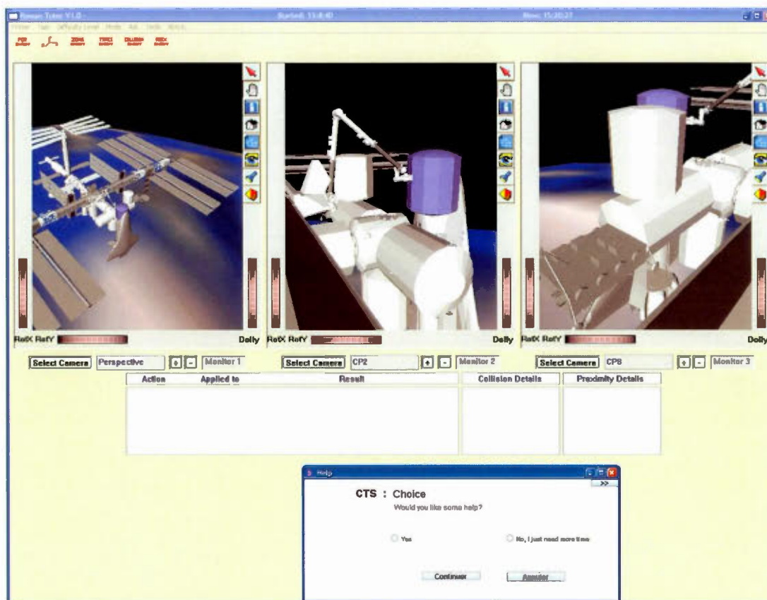
Figure 37 When CTS cannot think of a cause, it simply offers help (if the idea of intervening is not opposed during the deliberation). If the astronaut accepts, then choices are offered for selecting the help desired.
