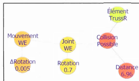
Figure 8 Portion of the "active" Perception Network. In this state, the network describes a rotation that brought joint WE to a distance of 6.96 from the Space Station element TrussR, creating a situation of possible collisions. Source: Hohmeyer (2006).
