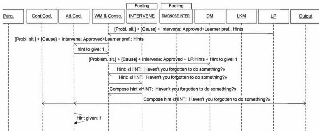
Figure 29 Selection and presentation of a hint to the user. An attention codelet keeps track of how many hints have been offered to the user.
