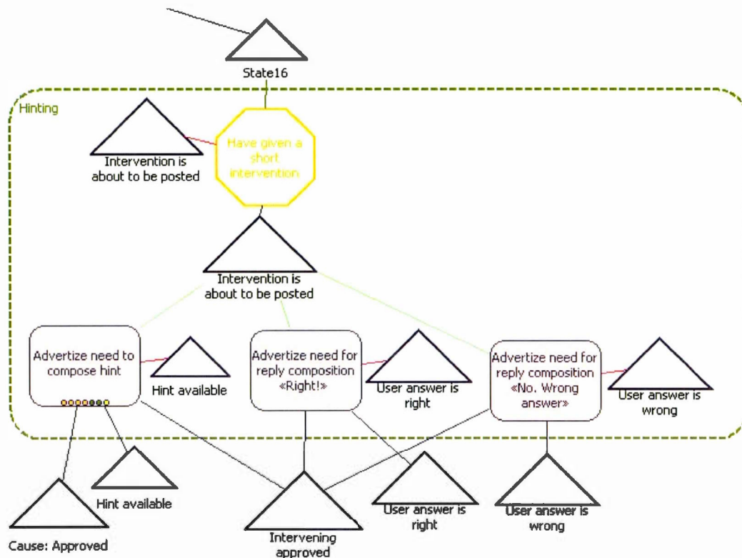
Figure 28 The Hinting stream of the BN. The context that renders hinting applicable is composed of three preconditions: «Intervening approved», «Cause approved» and «Hint available». Not showing here (above the stream) is the feeling it serves: «Need to intervene». When all the preconditions have been created, the behavior «Advertize need to compose hint» becomes executable and may fire if its activation is over the BN specified threshold, and is the most activated executable behavior in the BN. Little colored dots in the Behavior represent the codelets that implement the Behavior.
