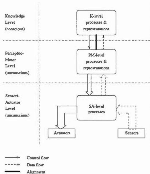
Figure 2 GLAIR's architecture.
